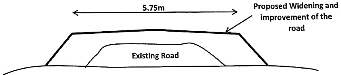
Cross Section of the Road
