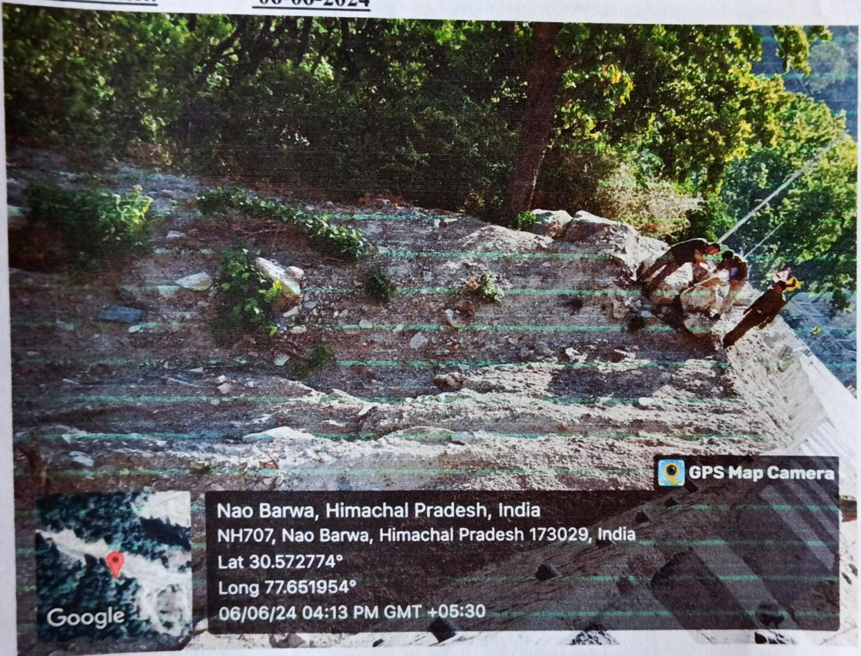
Dumping Site No.1 at RD 0/00 KM
