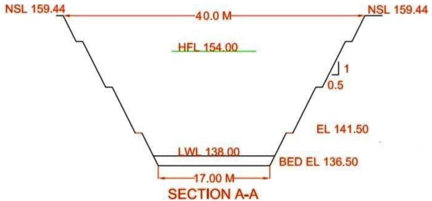
(TYPICAL SECTION OF CHANNEL)
