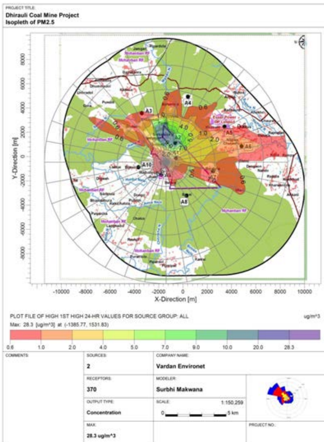
Figure 4.7: Controlled Condition Isopleths for 24 Hr. Incremental Conc. ( \mu\text{g}/\text{m}^3 ) for PM 2.5
