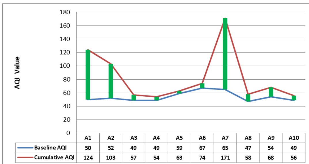
Figure 4.11: Comparison of AQI values with or without predicated GLC
