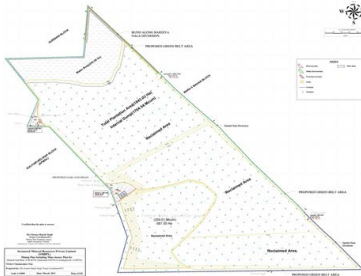
Figure 2.10: Mine Development Plan
