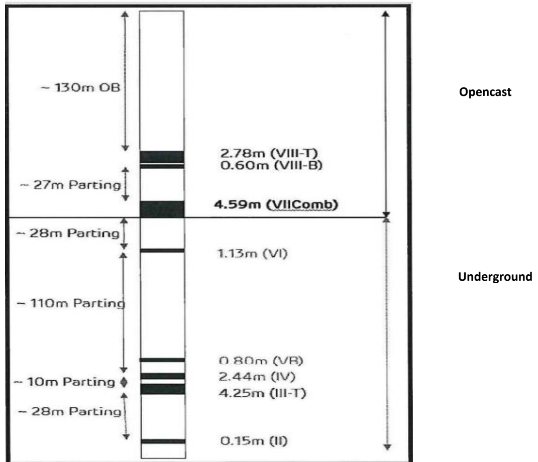
Figure 2.9: Generalized coal and Parting thickness
