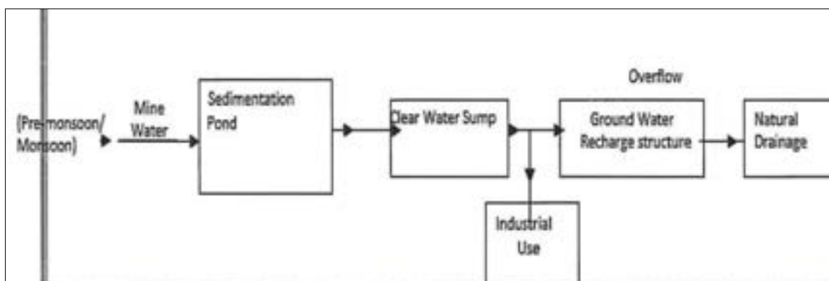
Figure 4.12: Mine water Treatment and Disposal
