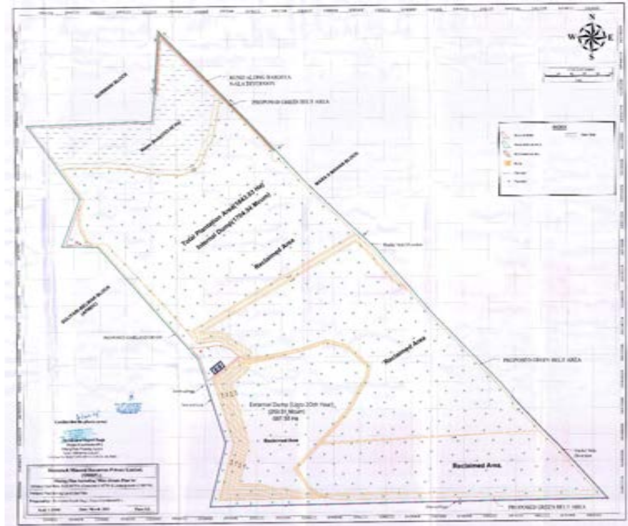
Figure 2.15: Post Mining Land Use Plan
