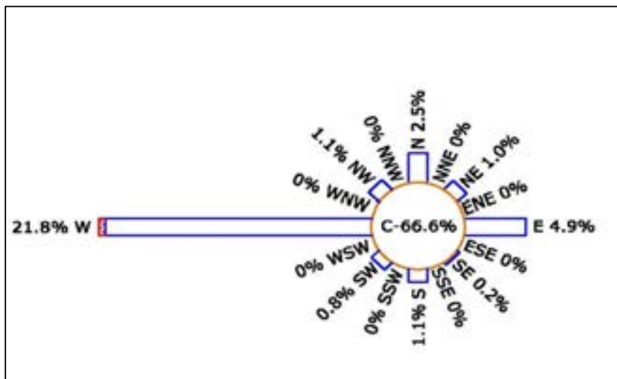
Figure 3.2: Wind Rose Diagram of Study Period (March to May 2021)
