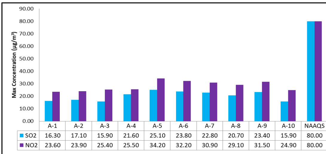
Figure 3.5: Graphical Representation of Gaseous Pollutants
