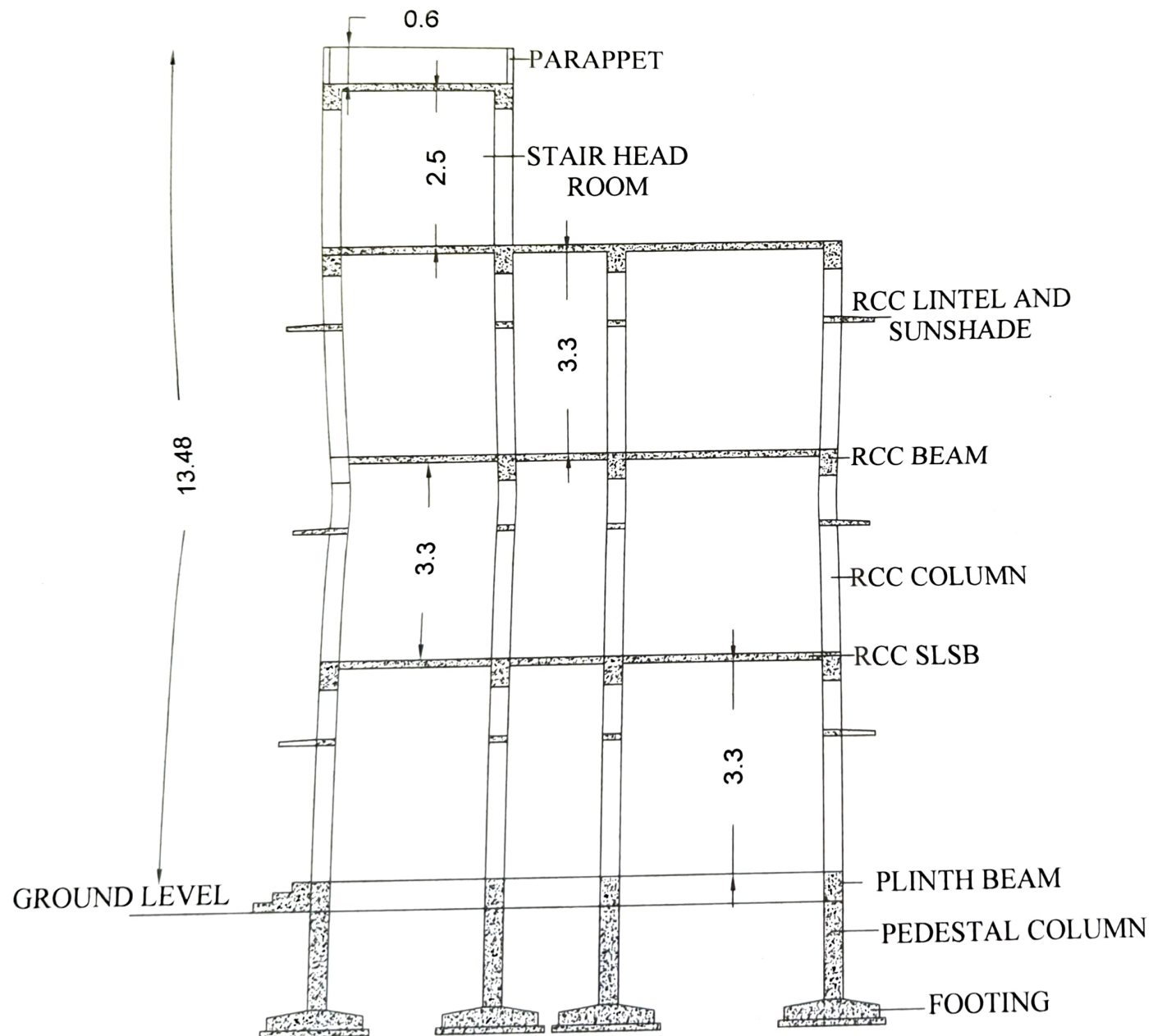
SECTION
