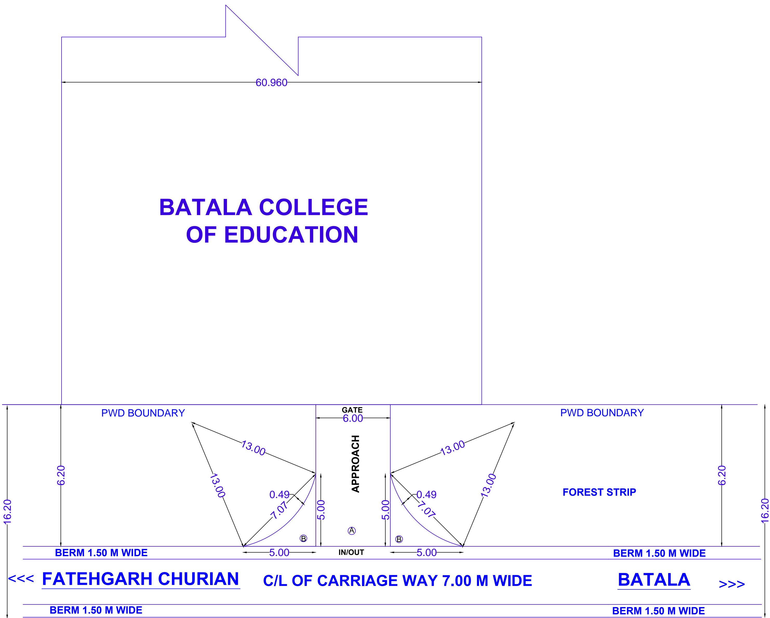
LAYOUT PLAN
