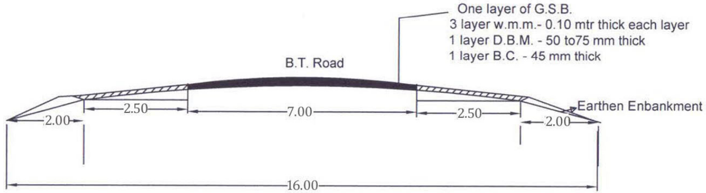
Cross-section of proposed road
