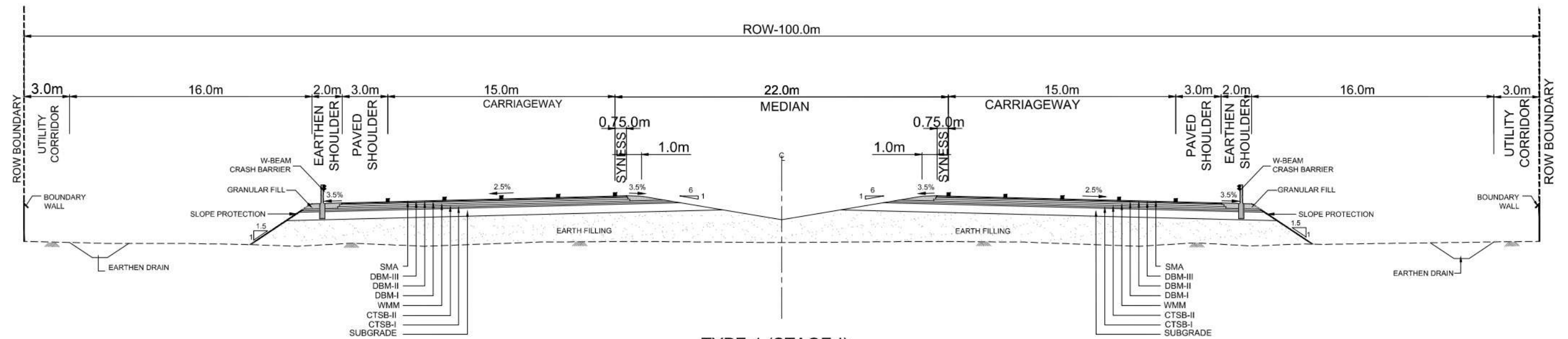
TYPE-1 (STAGE-I) TYPICAL CROSS SECTION FOR 8 LANE (2X4) IN PLAIN & ROLLING TERRAIN WITH DEPRESSED MEDIAN WITH EMBANKMENT HEIGHT UP TO 2.5 M.
