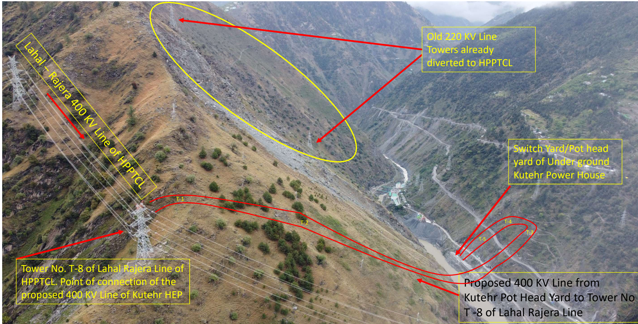
Kutehr 400 KV Transmission Line and Old 220KV Line Pic dtd. 20.04.2023
