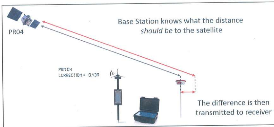
Fig. 4.5 Differential correction of error by DGPS
