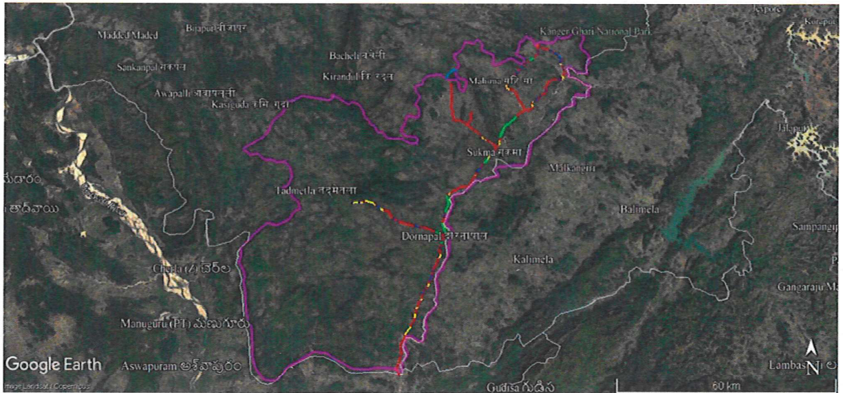
Fig-2: OFC Cable Proposed Routes on Satellite Imagery in Sukma Division.
