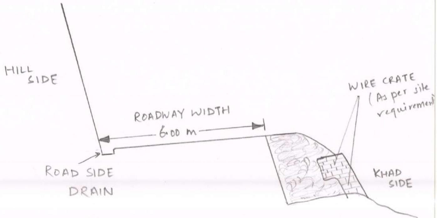
TYPICAL X-SECTION
