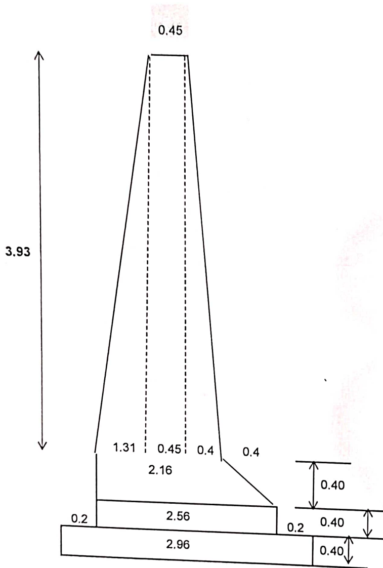
SECTION OF RETURN
