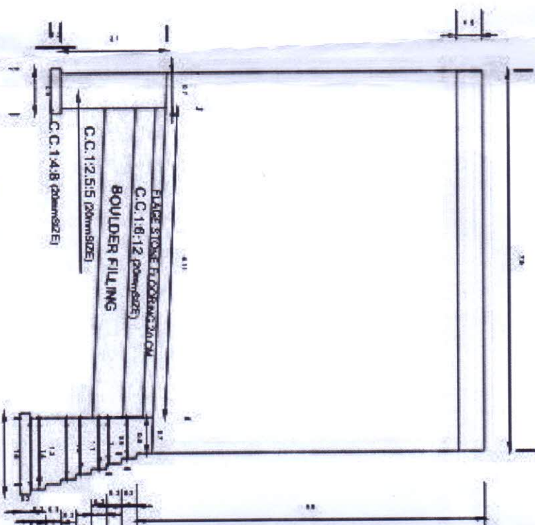
L-SECTION
