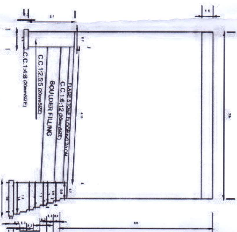
L-SECTION
