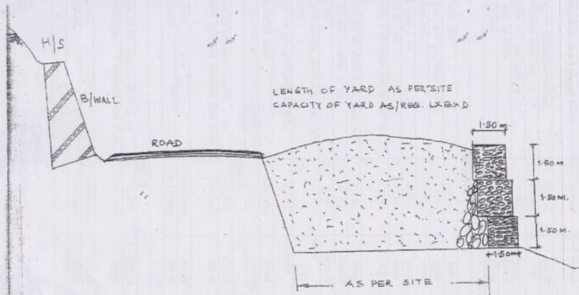
TYPICAL X-SECTION OF MUCK DISPOSAL YARD
