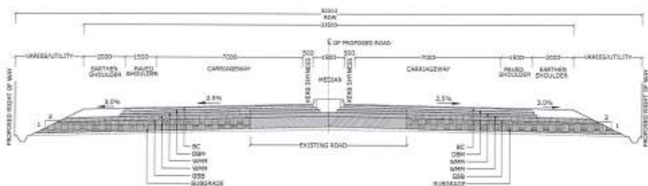
TCS-II TYPICAL CROSS SECTION FOR 4-LANE CONCENTRIC WIDENING ROAD IN PLAIN AND ROLLING TERRAIN
