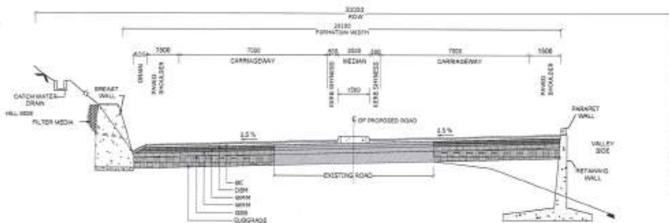
TCS-1 TYPICAL CROSS SECTION FOR 4-LANE CONCENTRIC WIDENING IN MOUNTAINOUS TERRAIN
