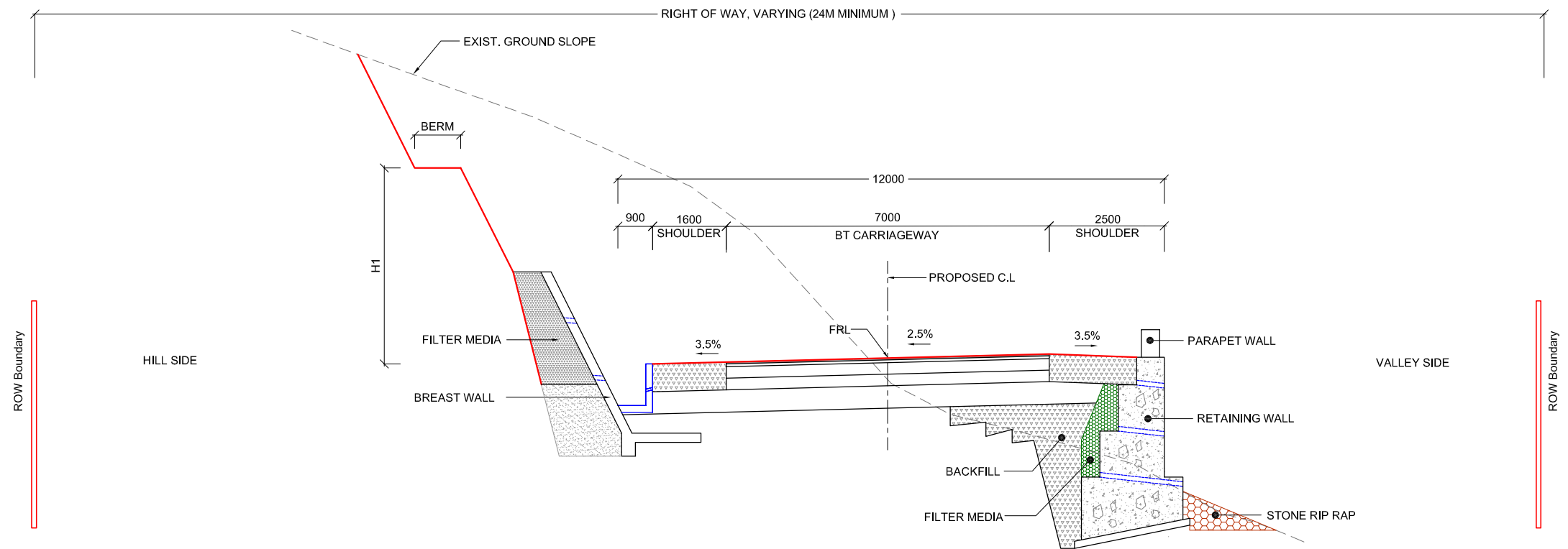
TCS IV - Typical Cross Section with Breast Wall on hill side and Retaining Wall on valley side
