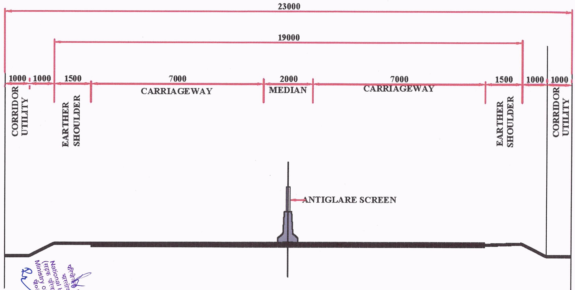
TCS 6A 4LANE ROAD IN FOREST SECTION (EMBANKMENT UP TO 1M)
