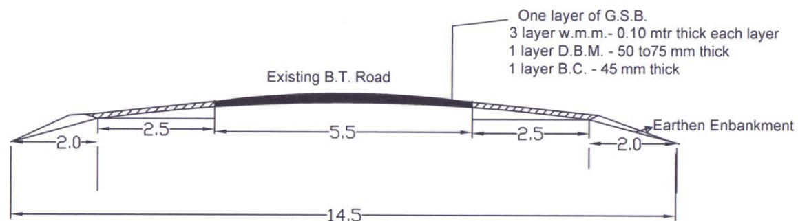
Cross-section of proposed road
