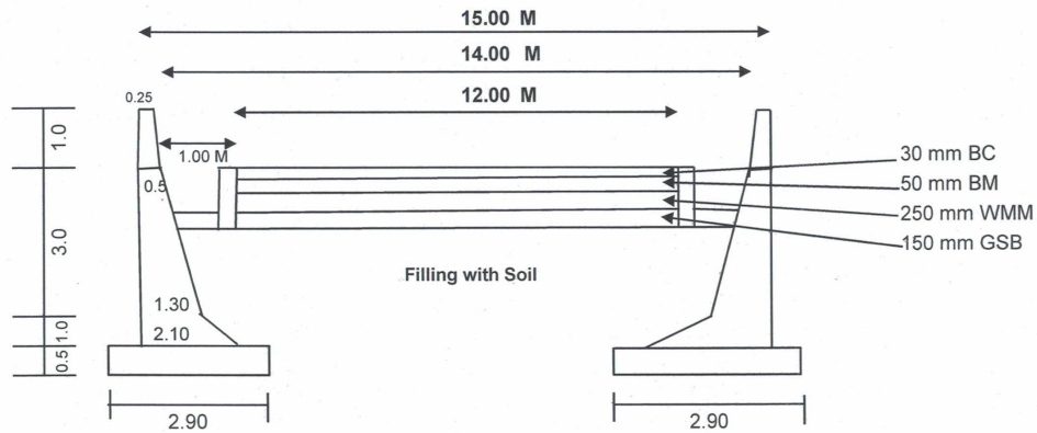
Typical Cross Section @ Km 520 for VCC 3.0 M Retaining wall and Filling with Soils inbetween Retaining Walls
