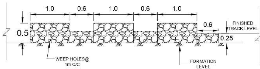
VALLEY SIDE ELEVATION
