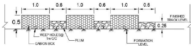
VALLEY SIDE ELEVATION
