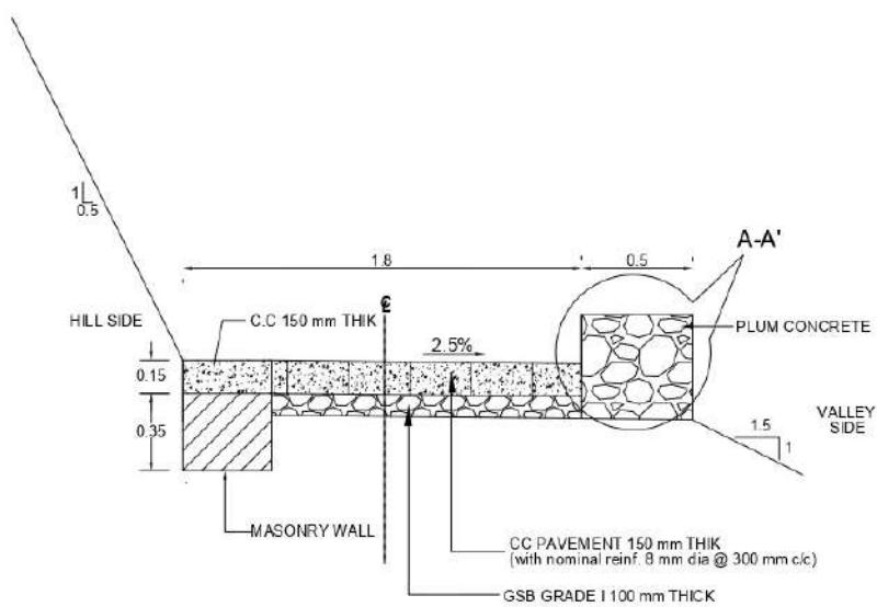
CROSS SECTION
