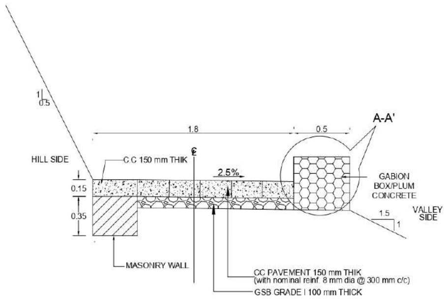
CROSS SECTION
