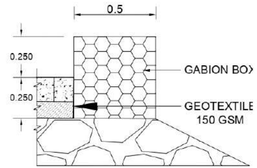
DETAIL A-A'
