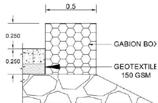
DETAIL A-A'
