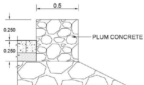
DETAIL A-A'
