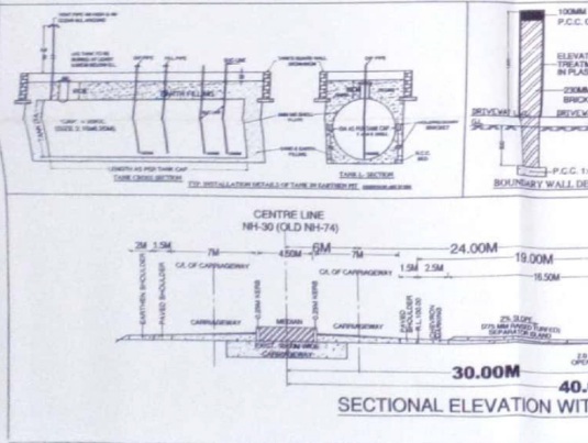
SECTIONAL ELEVATION WITH RESPECT TO NH (SECTION AT A - A) SCALE: 1:200
