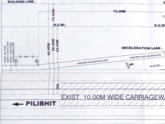
FUEL STATION LAY OUT PLAN SCALE: 1:300
