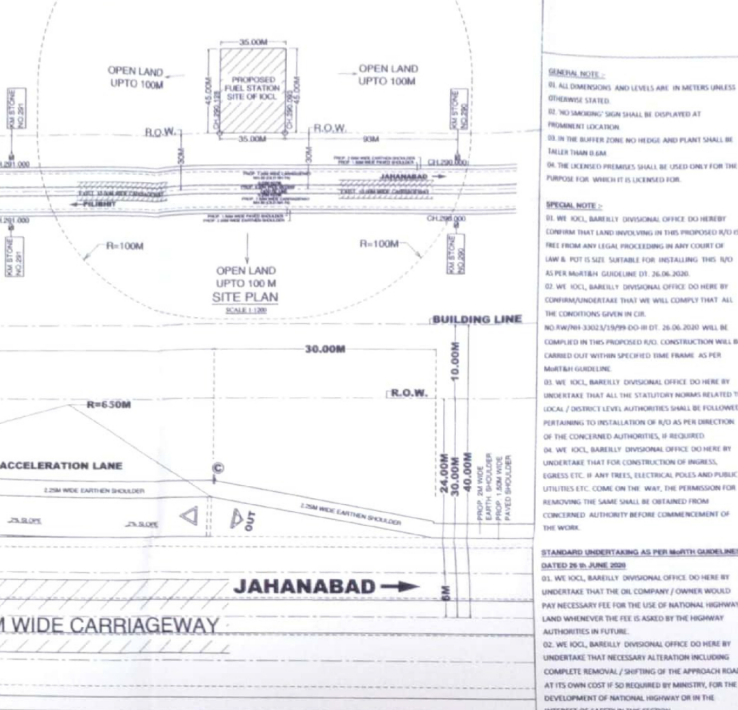
FUEL STATION LAY OUT PLAN SCALE: 1:300
