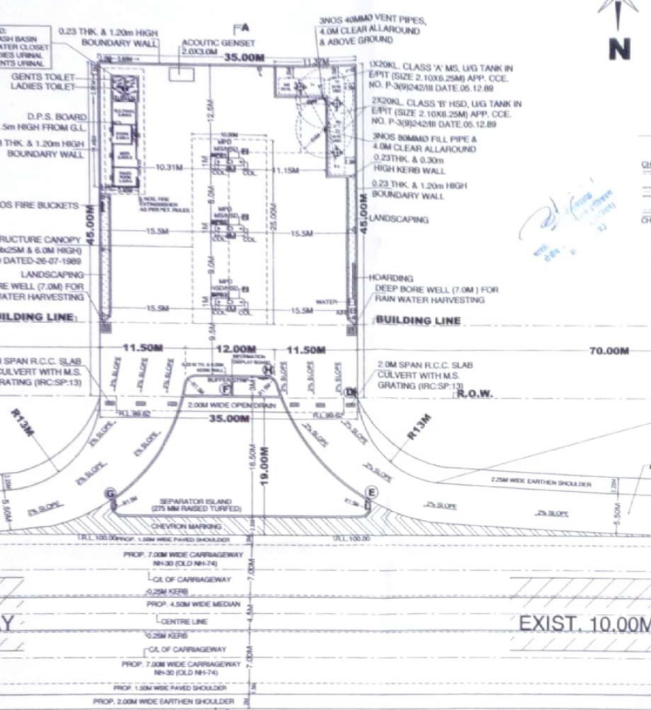
FUEL STATION LAY OUT PLAN SCALE: 1:300
