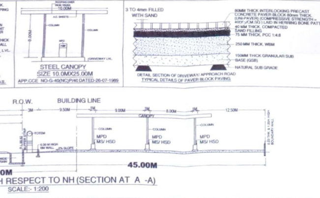
SECTIONAL ELEVATION WITH RESPECT TO NH (SECTION AT A - A) SCALE: 1:200
