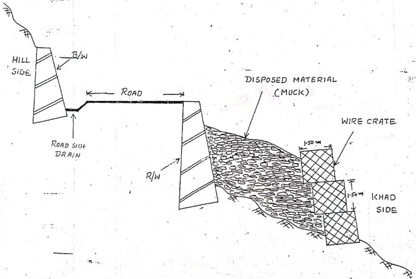
TYPICAL X-SECTION OF MUCK DISPOSAL PLAN
