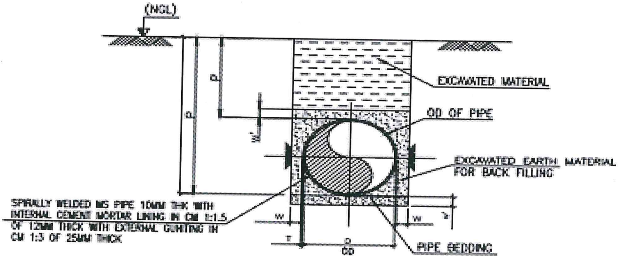
TYPICAL CROSS SECTION OF PIPELINE TRENCHES
