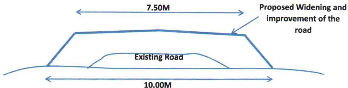
Cross Section of the Road
