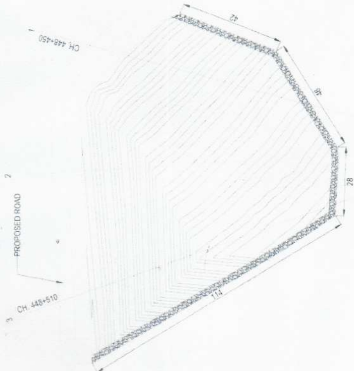
MUCK DISPOSAL AREA AT CH. 448+450 TO 448+510 SCALE 1:1000
