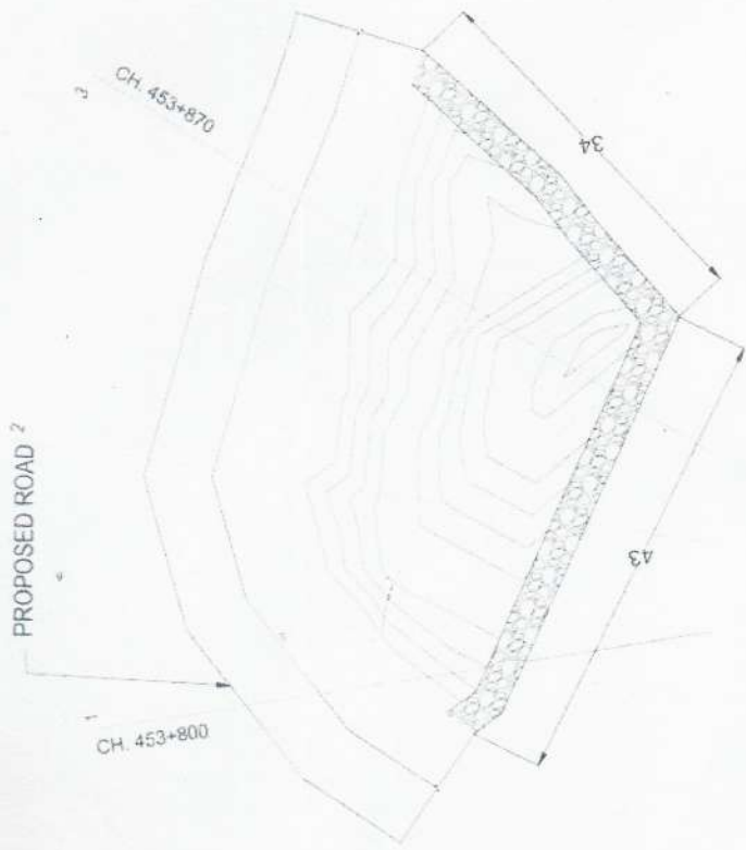
MUCK DISPOSAL AREA AT CH. 453+800 TO 453+870 SCALE 1:500
