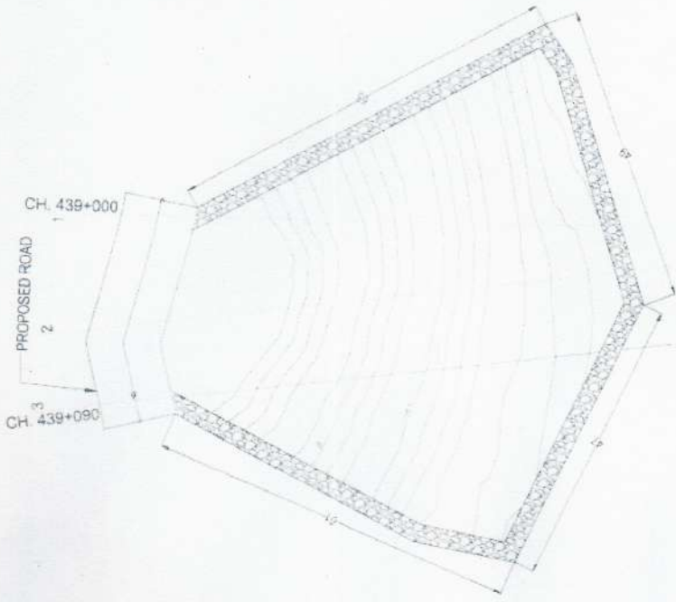
MUCK DISPOSAL AREA AT CH. 439+000 TO 439+090 SCALE 1:750
