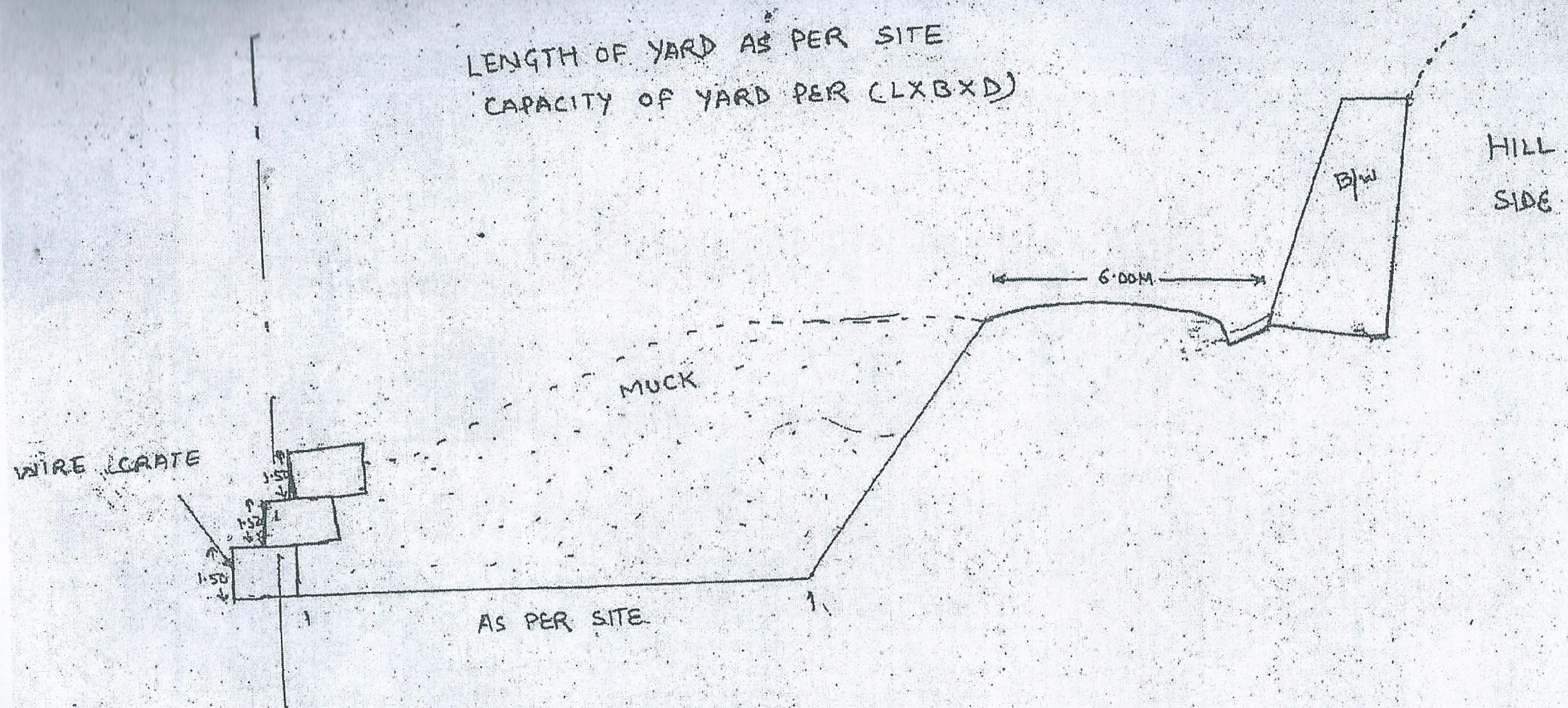
TYPICAL SECTION OF MUCK DISPOSAL YARD
