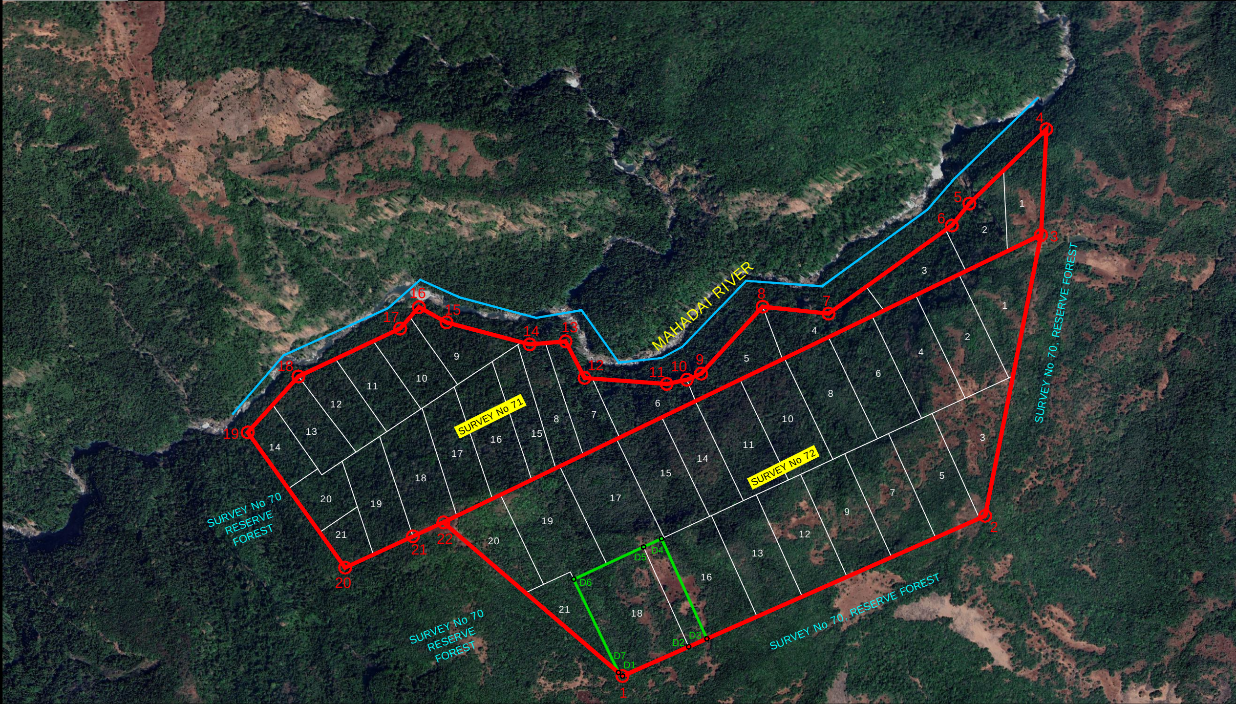
GPS READINGS OF SURVEY No 71 & 72 OF GAVALI VILLAGE, KHANAPUR TALUK
