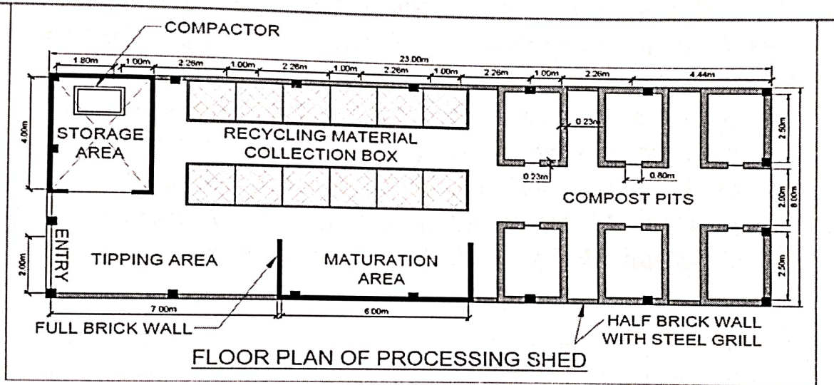
Fig. Layout of the tipping & plastic segregation shed
