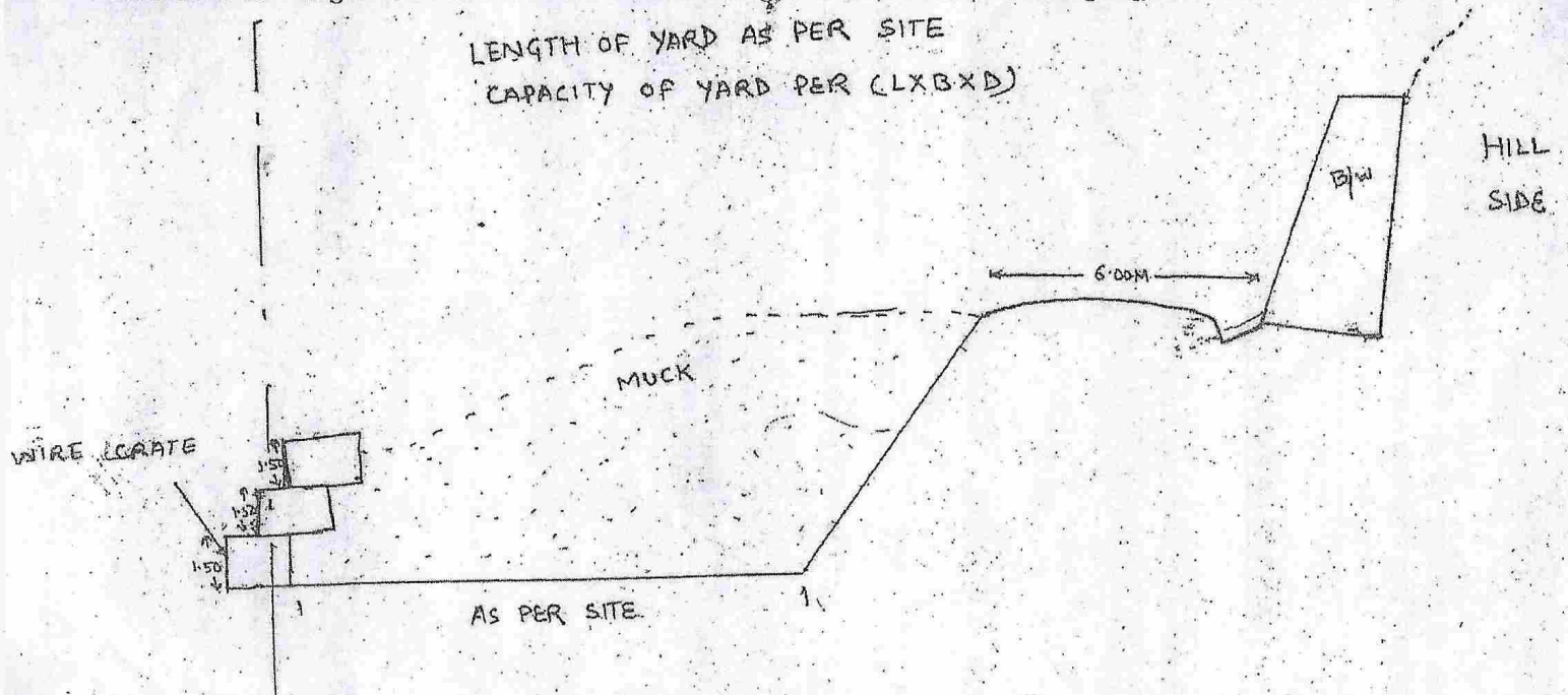
TYPICAL SECTION OF MUCK DISPOSAL YARD
