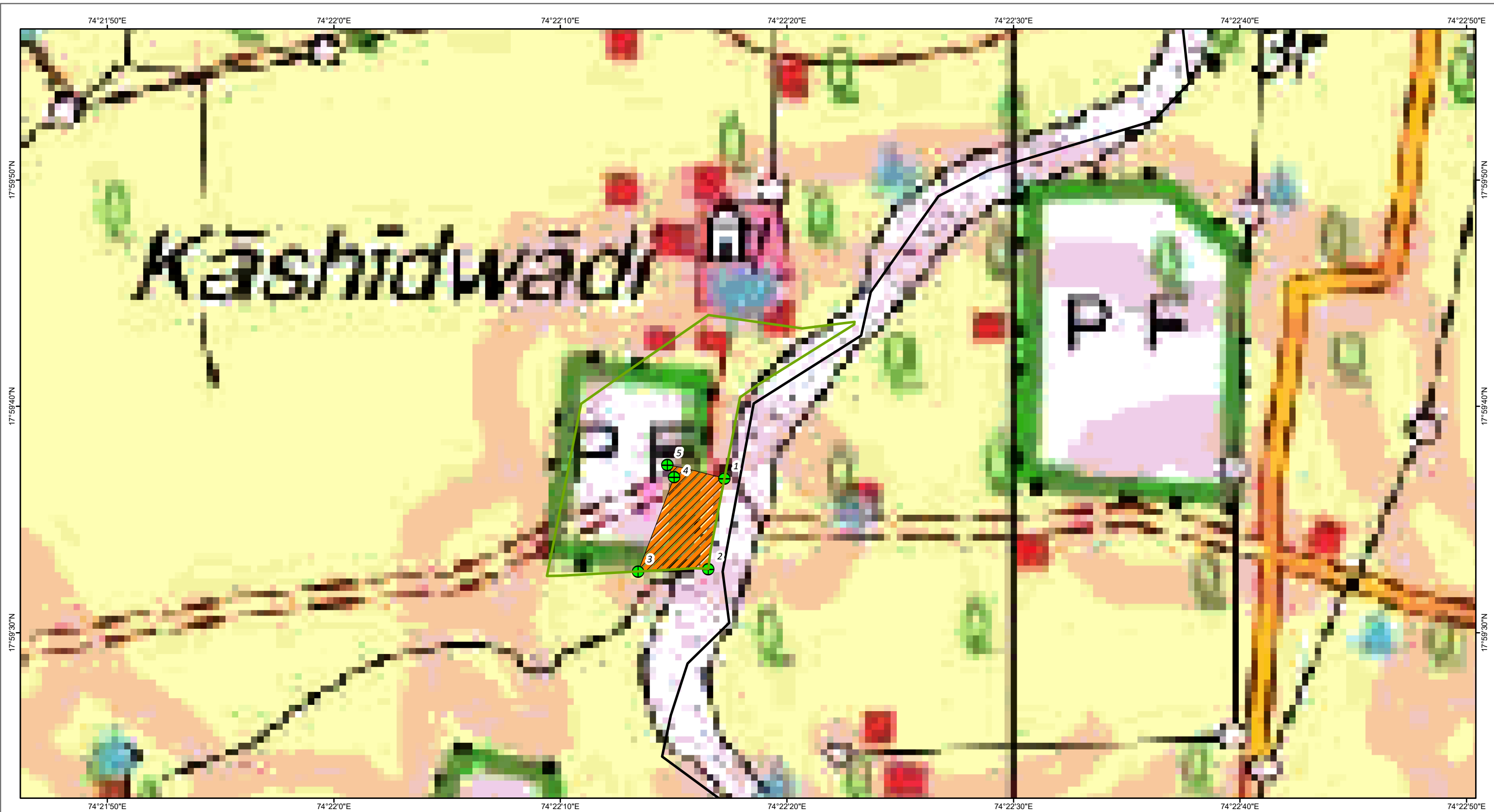
1:50000 SOI TOPOSHEET INDICATING DIVERSION OF FOREST LAND FOR UNDERGROUND OFC DUCT AND CABLE WITHIN ROW OF EXISTING ROAD SH – 13, ROAD PASSING THROUGH FOREST LAND AT PALASHITAL- MAAN DIST – SATARA PROPOSAL UNDER FOREST (CONSERVATION) ACT 1980
