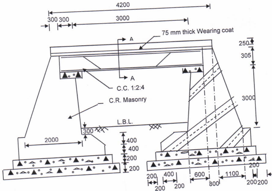
CROSS SECTION
