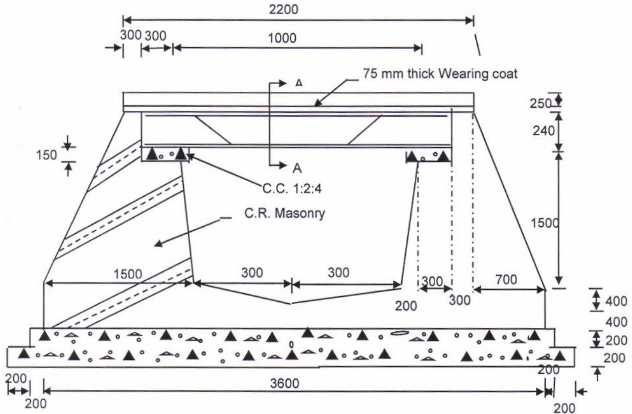
CROSS SECTION
