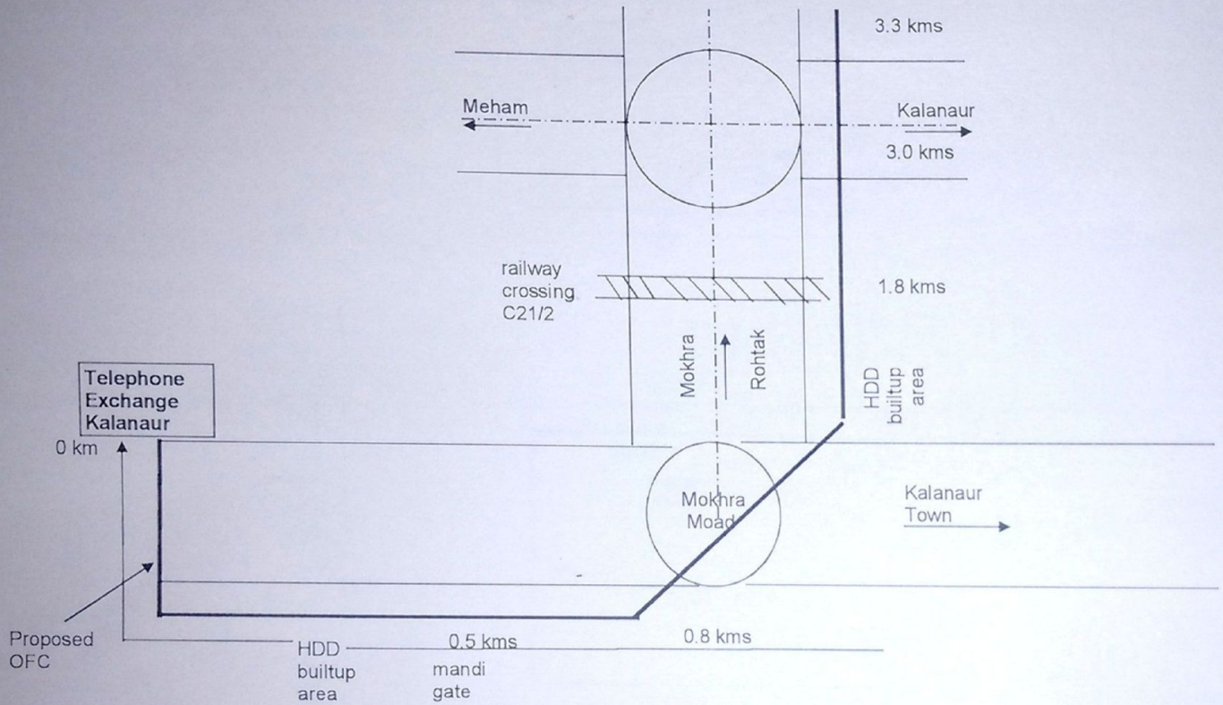
Route Diagram For Kalanaur TE - Rohtak TE 24F OF Cable
