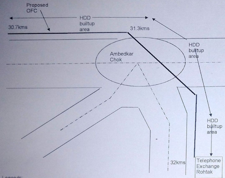
Route Diagram For Kalanaur TE - Rohtak TE 24F OF Cable
