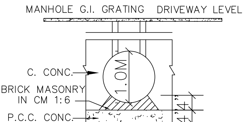
1.0M DIA DETAIL OF DRAINAGE RAIN WATER PIPE
