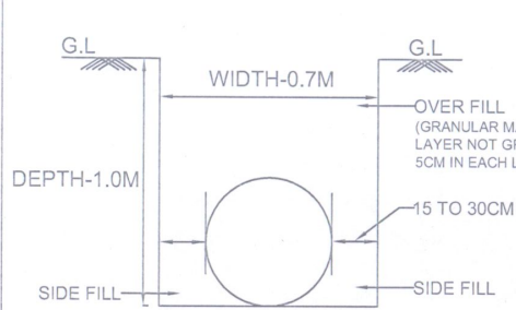
HDPE PIPE DETAIL (63 MM TO 140MM)
