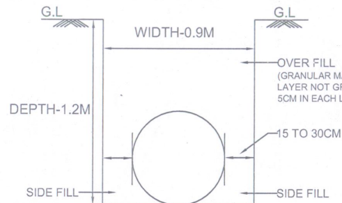
HDPE PIPE DETAIL (160 MM TO 250MM)
