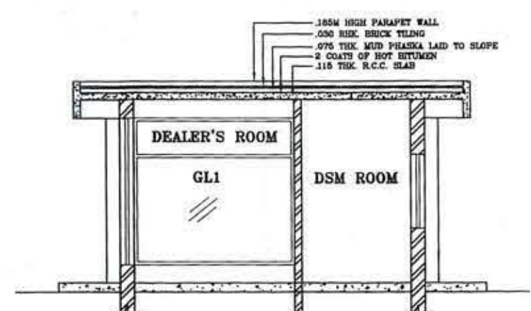
SECTION B-B
