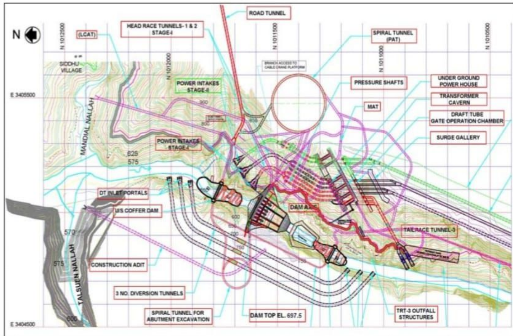
Figure 2.1: Layout map of Sawalkote H.E. Project (Source: DPR Sawalkote HEP)
