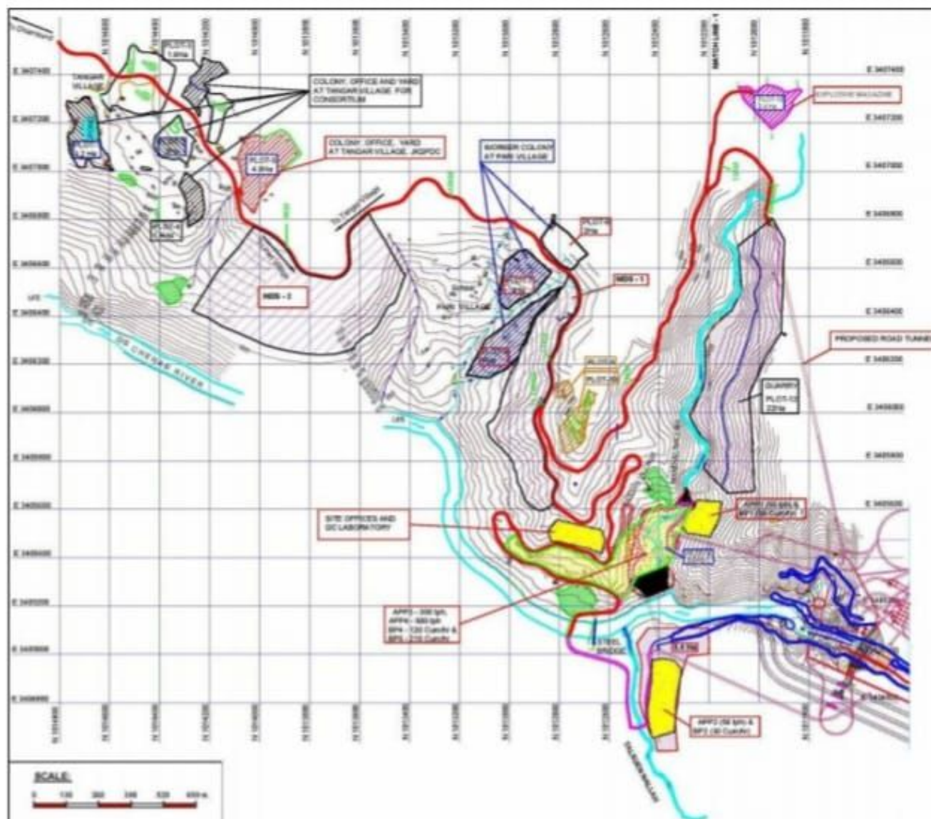
Figure 2.2: Layout map construction facilities area of Sawalkote H.E. Project (Source: DPR Sawalkote HEP)
