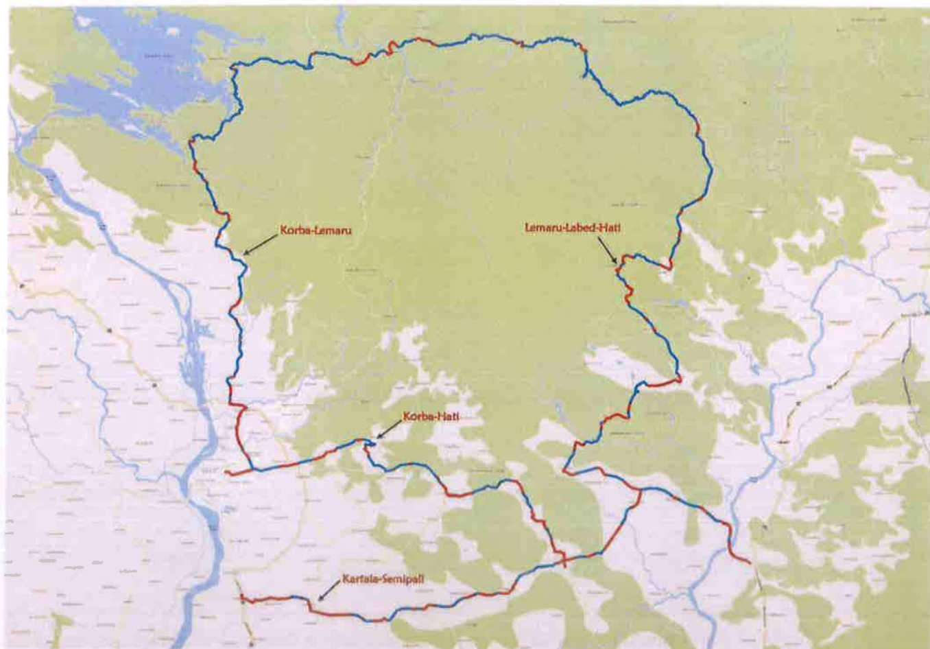
Fig-1: OFC Cable Proposed Routes on Online Map in Korba Division.
