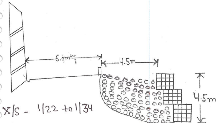
X-SECTION
