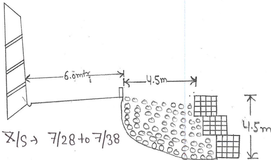
X-SECTION
