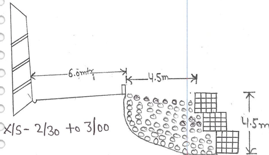
X-SECTION
