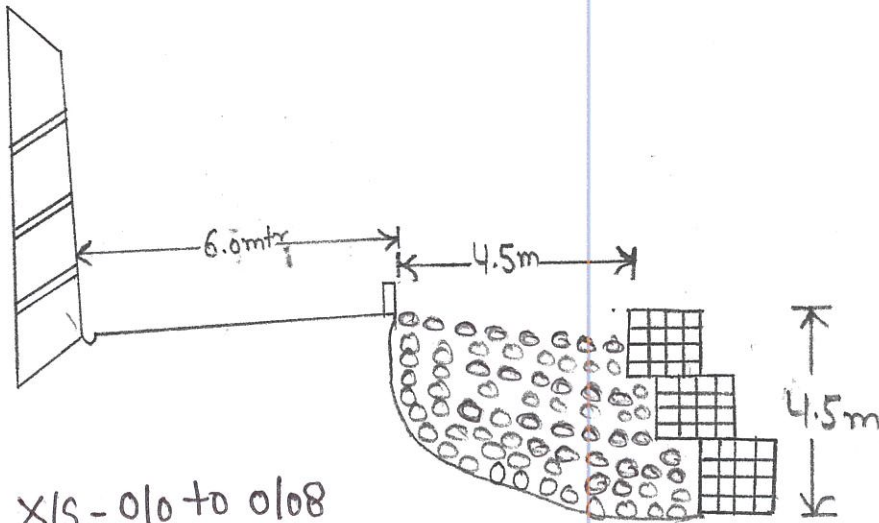
X - SECTION
