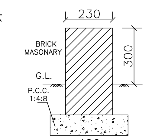
DETAILS OF KERB WALL (KW)
