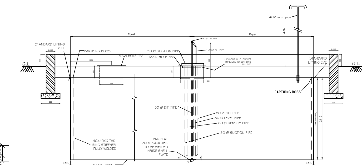
LONGITUDINAL PART ELEVATION PART SECTION
