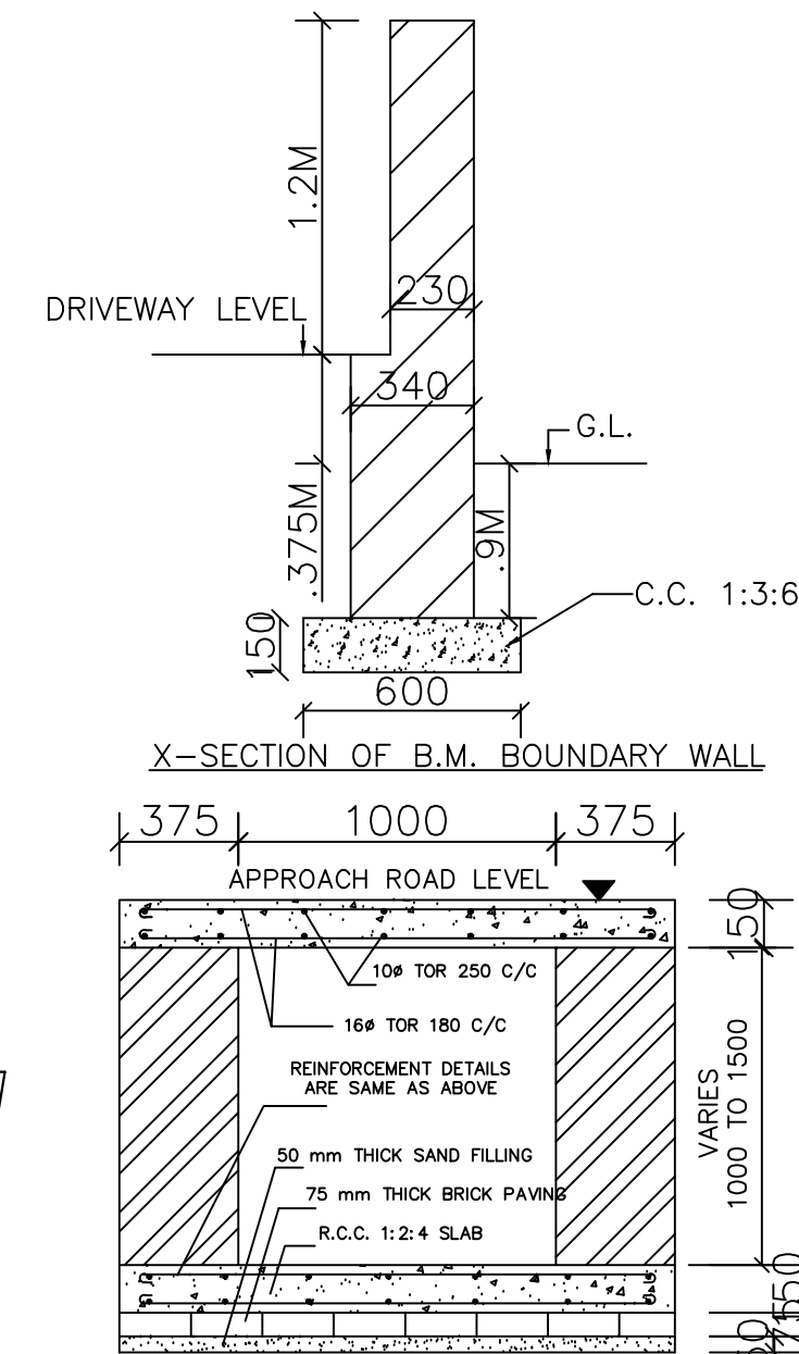
CROSS SECTION OF CULVERT DESIGN AS PER IRC:SP-13 (TYPE-A)
