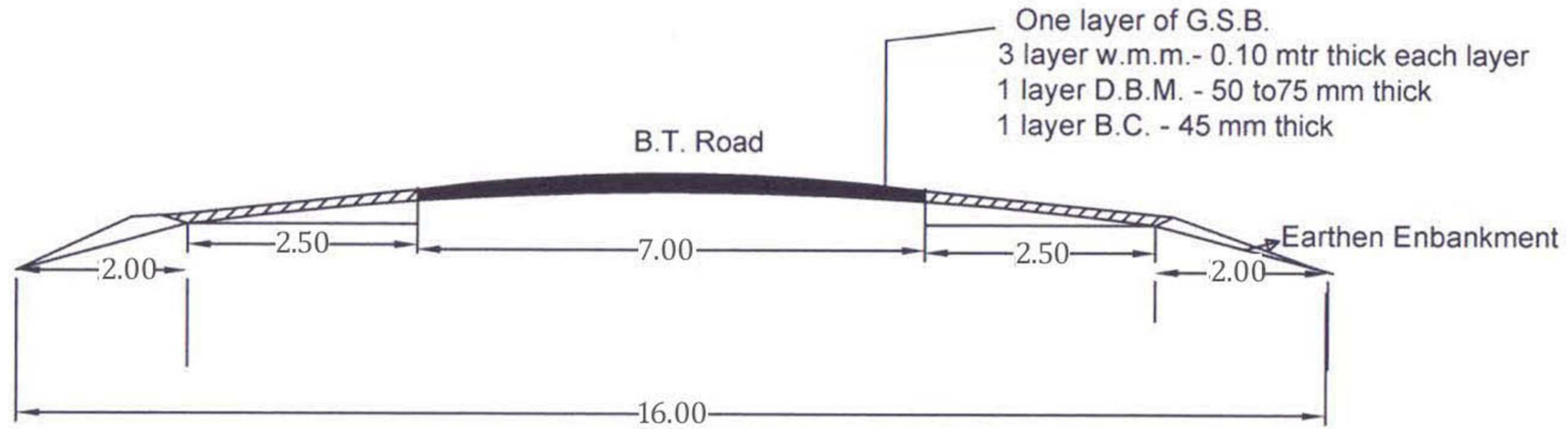
Cross-section of proposed road
