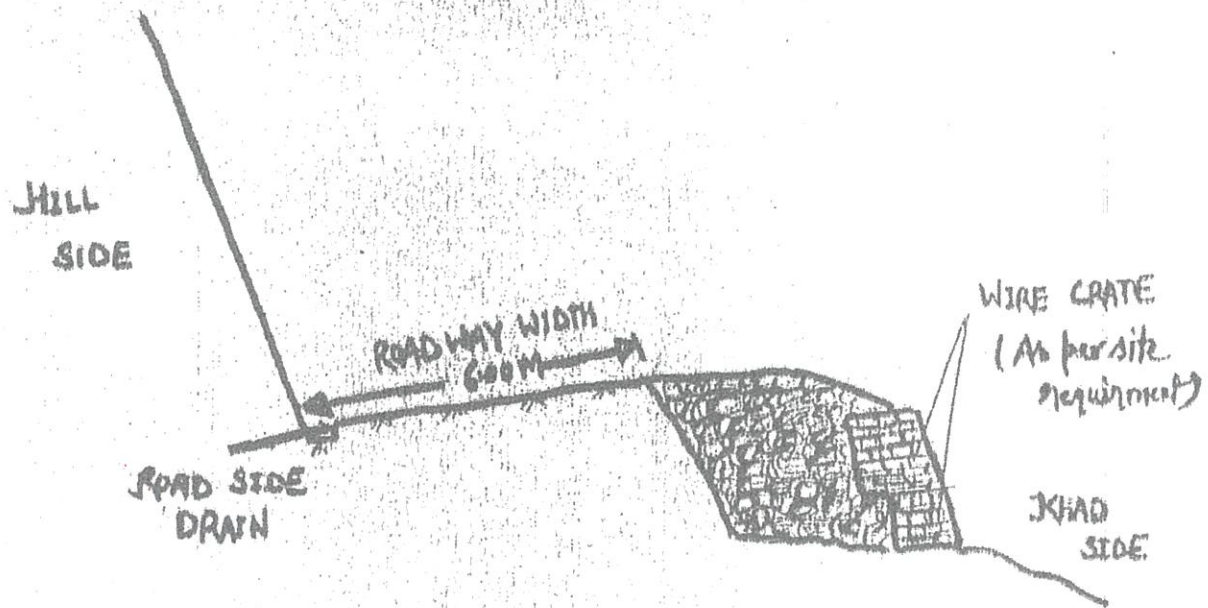
TYPICAL X-SECTION
