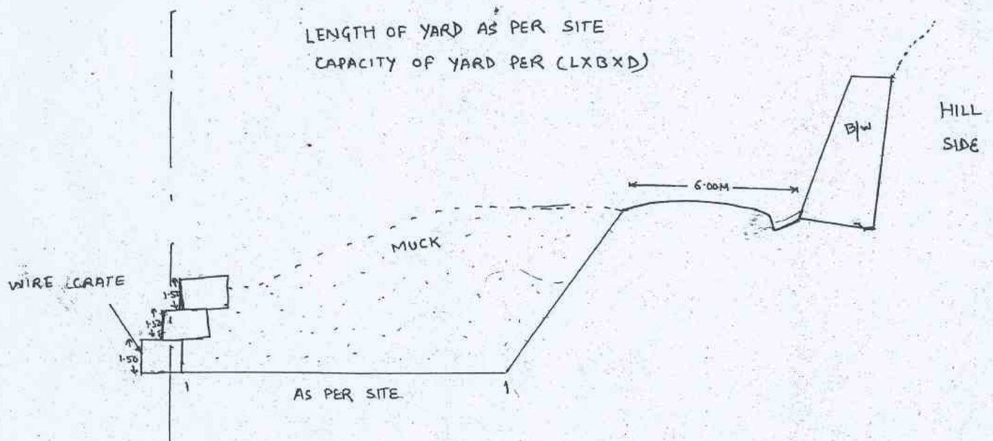
TYPICAL SECTION OF MUCK DISPOSAL YARD
