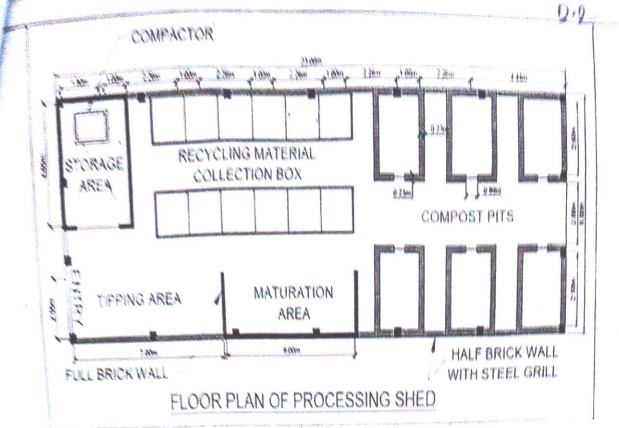
Fig. Layout of the tipping & plastic segregation shed
