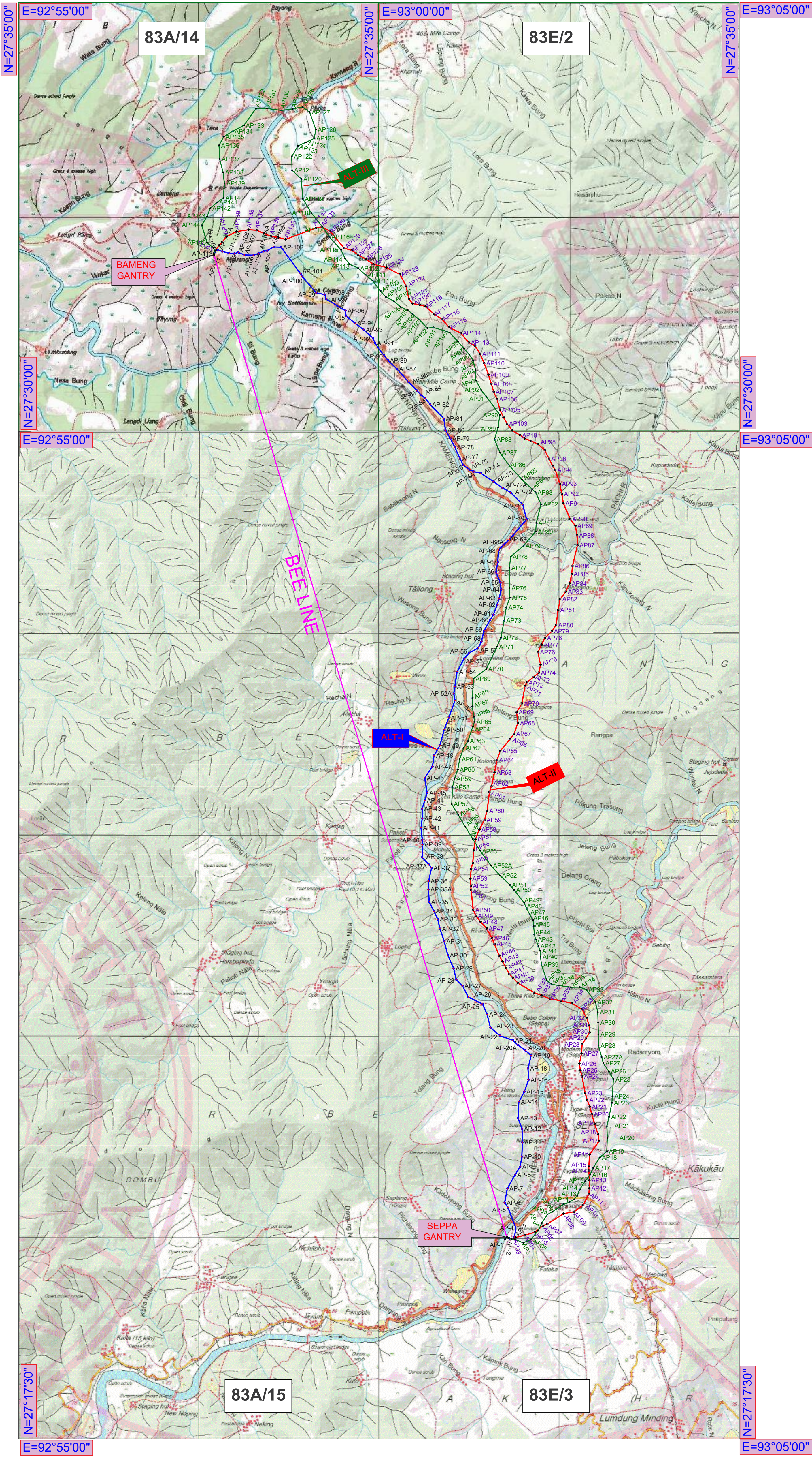
Three Alternative Route of 132KV S/C(on D/C TOWER) SEPPA-BAMENG TRANSMISSION LINE Package No-TW24
