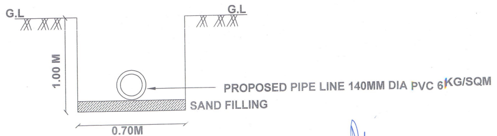
CROSS SECTION OF PIPE LINE
