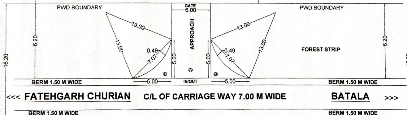
LAYOUT PLAN
