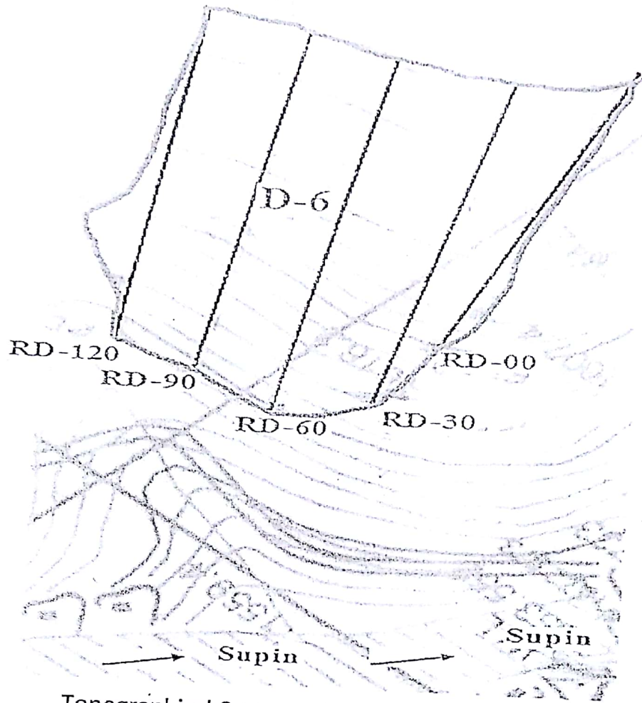
Topographical Contour Map of Dumping Site-6 (D-6)
