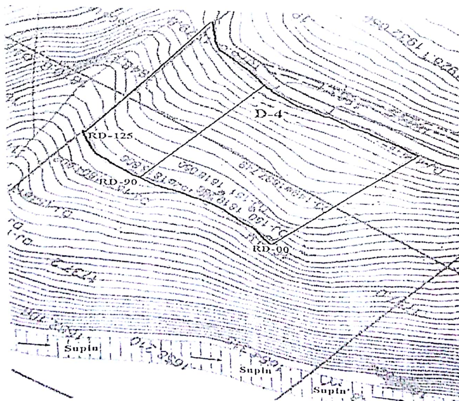
Topographical Contour Map of Dumping Site-4 (D-4)
