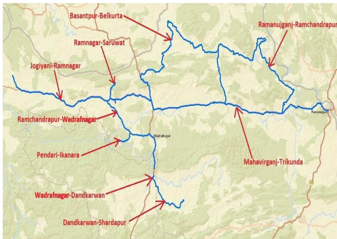
Fig-1.1: Segment-I , OFC Cable Proposed Routes on Online Map in Balrampur Division.
