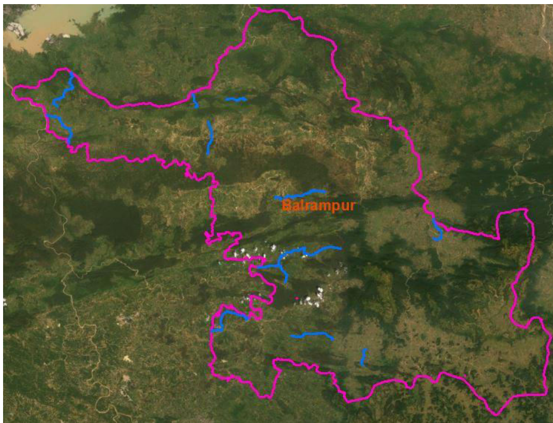
Fig-2.3: Segment-III - OFC Cable Proposed Routes on Satellite Imagery in Balrampur Division.
