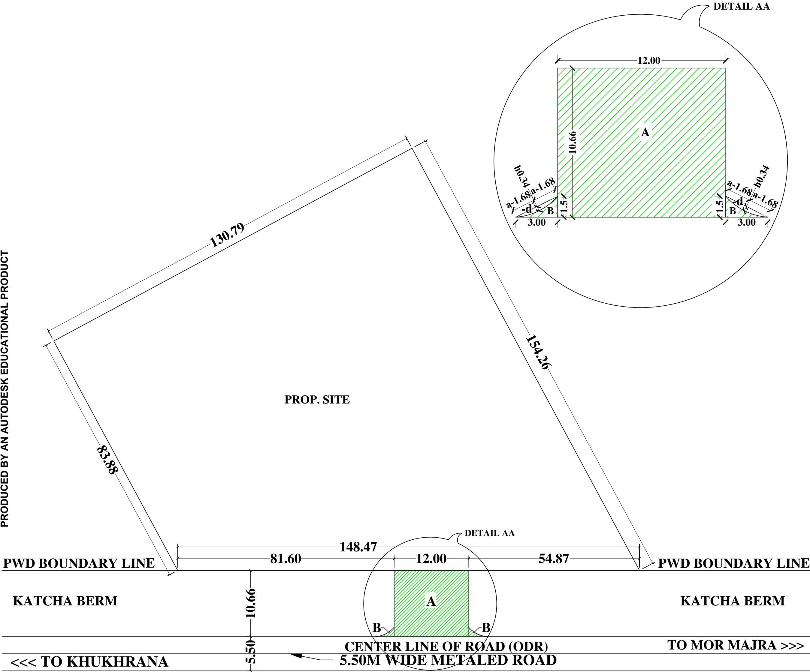
LAYOUT PLAN
